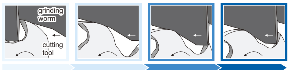
Fig. 2 Engagement conditions near the cutting edge during continuous generating grinding of cutting tools [21]
